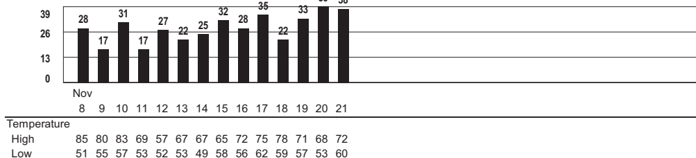
DAILY KWH USAGE FOR BILLING PERIOD
